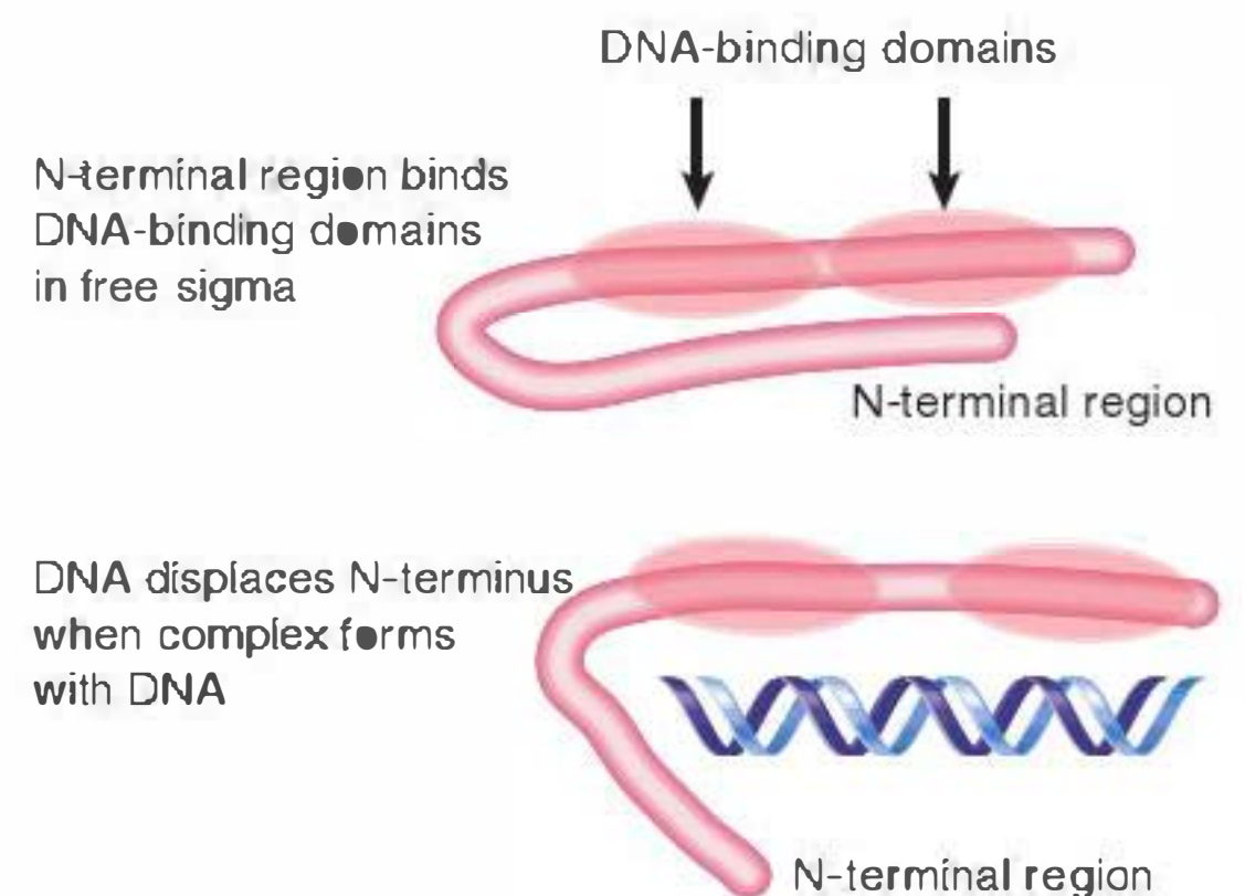
FIGURE 19.18 The N-terminus of sigma blocks the DNA-binding regions from binding to DNA. When an open complex forms, the N-terminus swings 20 Å away, and the two DNA-binding regions separate by 15 Å.
