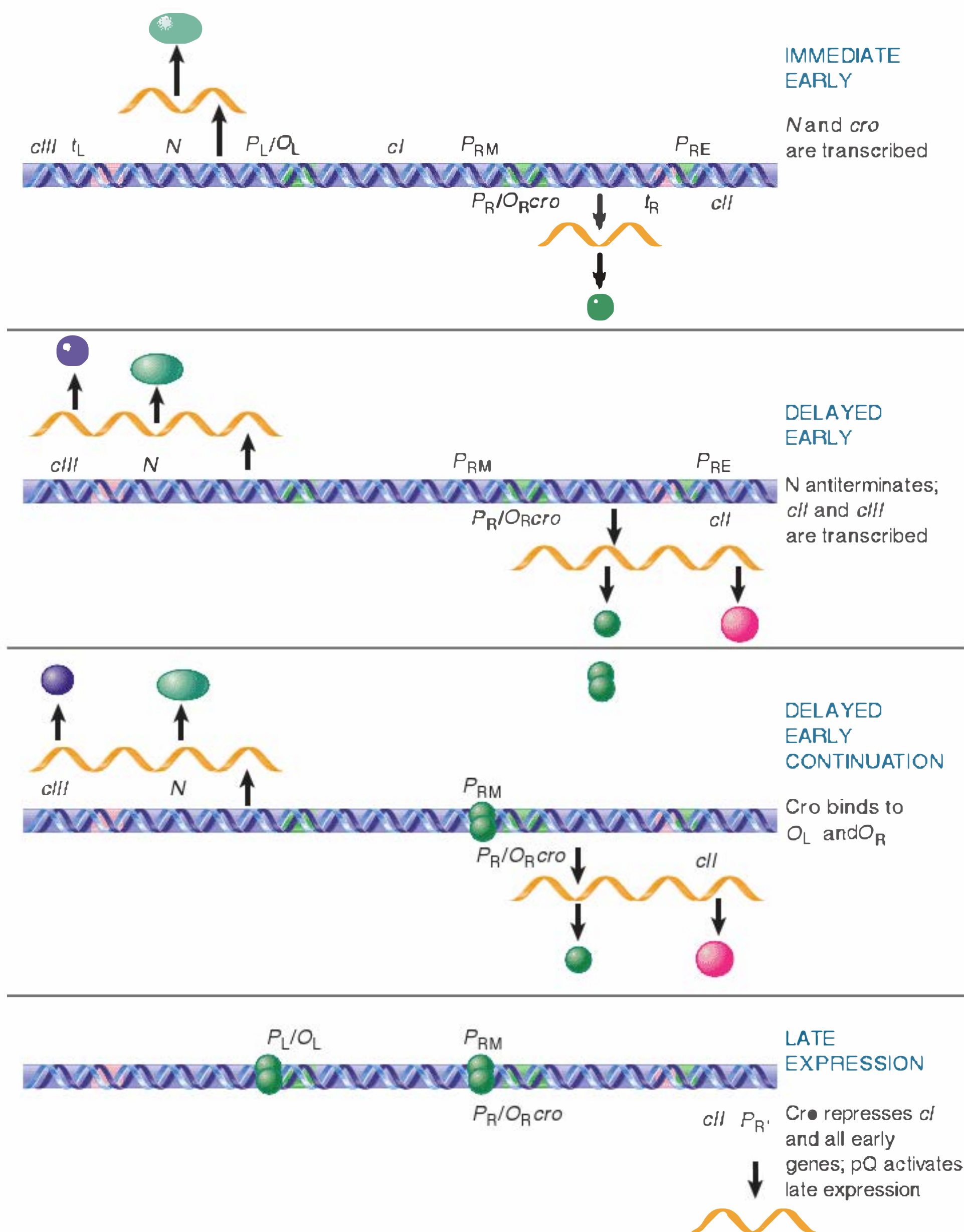
FIGURE 27.34 The lytic cascade requires Cro protein, which directly prevents repressor maintenance via P_{RM} , as well as turning off delayed early gene expression, indirectly preventing repressor establishment.
