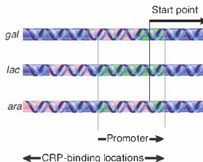
FIGURE 26.30 The CRP protein can bind at different sites relative to RNA polymerase.
