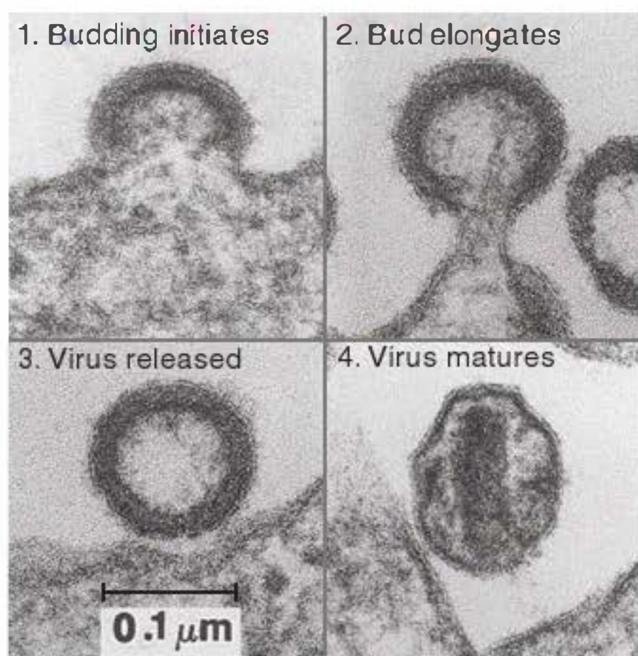
FIGURE 17.22 Retroviruses (HIV) bud from the plasma membrane of an infected cell. Photos courtesy of Matthew A. Gonda, Ph.D., Partner at Power Ten Medical Ventures, Inc.
