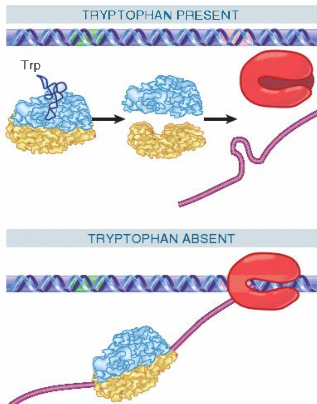
FIGURE 26.38 In the presence of tryptophan tRNA, ribosomes translate the leader peptide and are released. This allows hairpin formation, so that RNA polymerase terminates. In the absence of tryptophan tRNA, the ribosome is blocked, the termination hairpin cannot form, and RNA polymerase continues.
