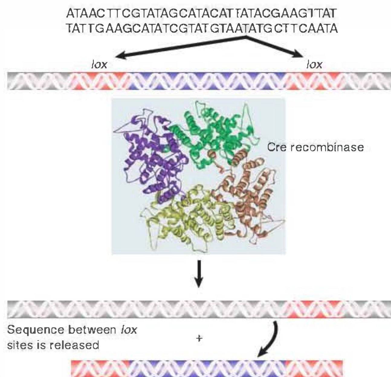
FIGURE 3.31 The Cre recombinase catalyzes a site-specific recombination between two identical lox sites, releasing the DNA between them. Structure from Protein Data Bank: 1OUQ. E. Ennifar, et al., Nucleic Acids Res. 31 (2003): 5449–5460.
