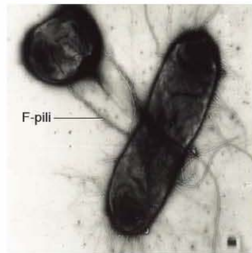
FIGURE 14.10 Mating bacteria are initially connected when donor F-pili contact the recipient bacterium. Photo courtesy of Emeritus Professor Ron Skurray, School of Biological Sciences, University of Sydney.
