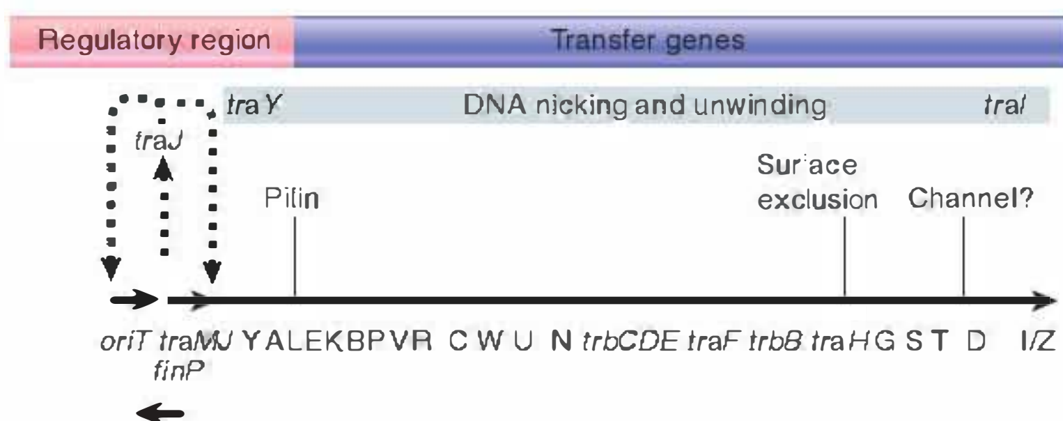
FIGURE 14.9 The tra region of the F plasmid contains the genes needed for bacterial conjugation.
