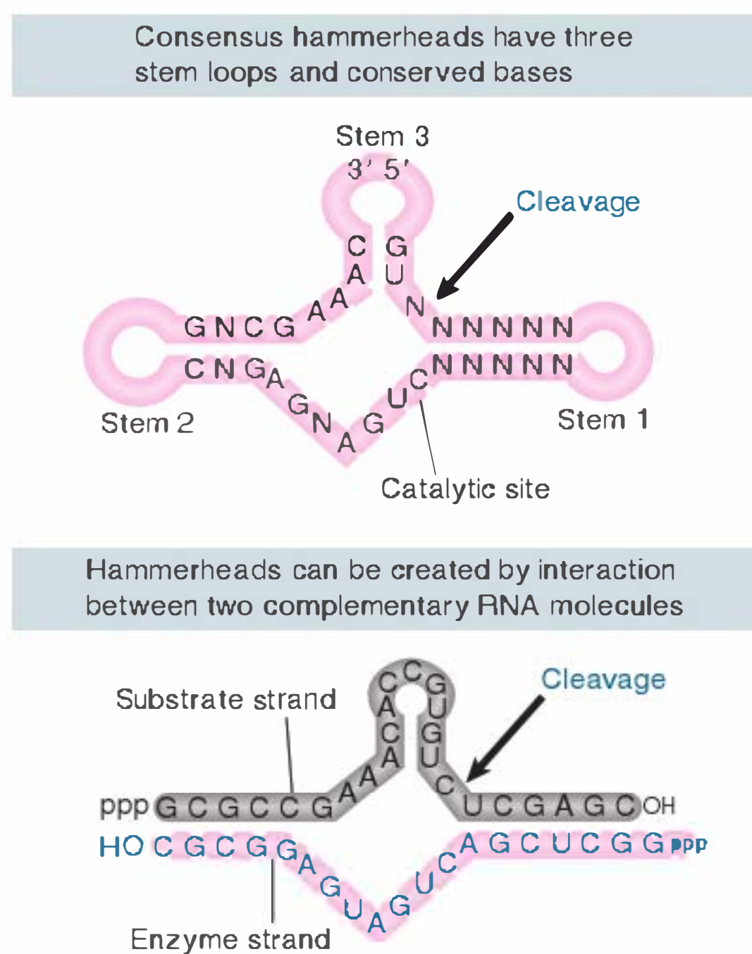
FIGURE 23.14 Self-cleavage sites of viroids and virusoids have a consensus sequence and form a hammerhead secondary structure by intramolecular pairing. Hammerheads can also be generated by pairing between a substrate strand and an “enzyme” strand. The three loop regions at the end of the stems are optional.
