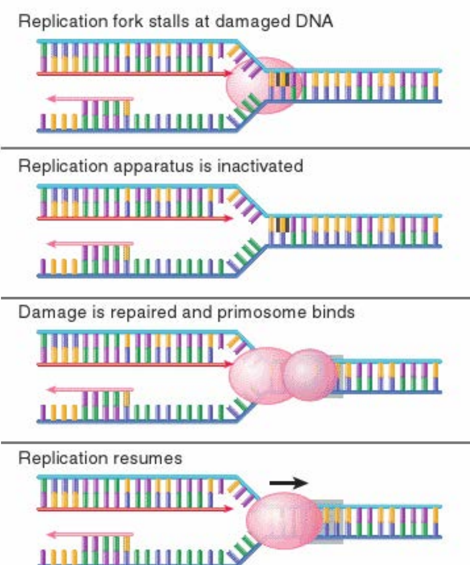
FIGURE 13.29 The primosome is required to restart a stalled replication fork after the DNA has been repaired.
