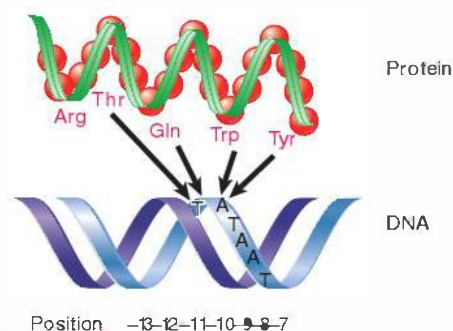
FIGURE 19.17 Amino acids in the 2.4 \alpha -helix of \beta^{70} contact specific bases in the coding strand of the -10 promoter sequence.
