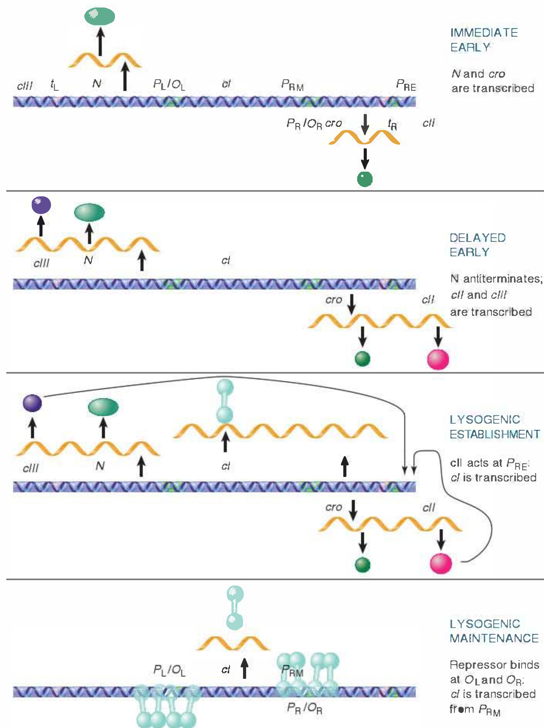
FIGURE 27.33 A cascade is needed to establish lysogeny, but then this circuit is switched off and replaced by the autogenous repressor-maintenance circuit.
