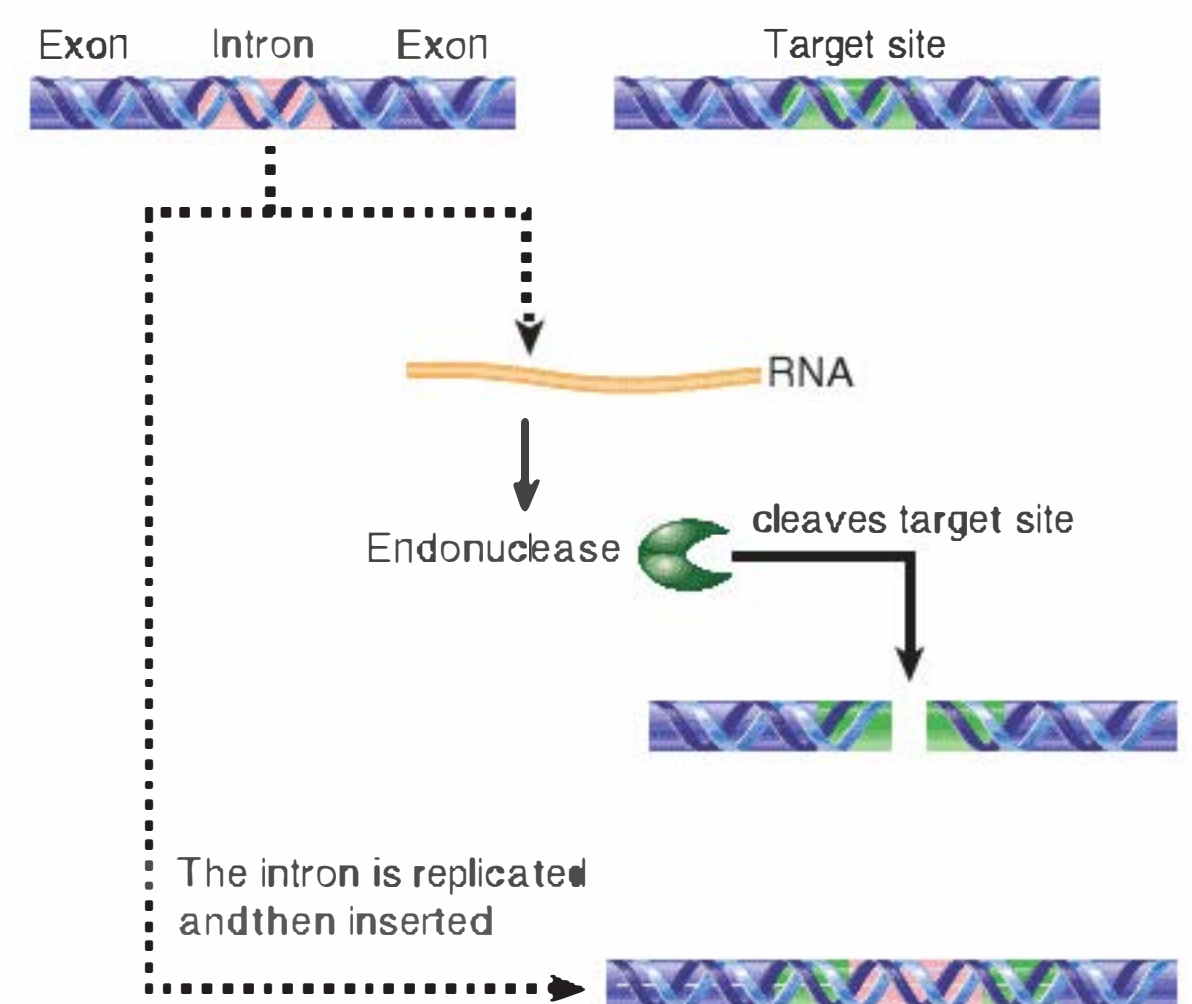
FIGURE 23.11 An intron encodes an endonuclease that makes a double-strand break in DNA. The sequence of the intron is duplicated and then inserted at the break.
