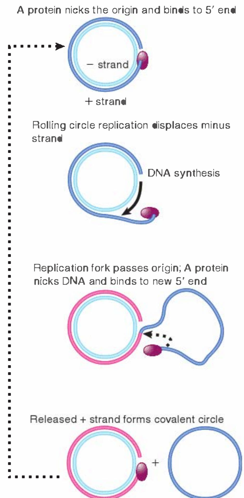
FIGURE 14.8 \Phi X174 RF DNA is a template for synthesizing single-stranded viral circles. The A protein remains attached to the same genome through indefinite revolutions, each time nicking the origin on the viral (+) strand and transferring to the new 5' end. At the same time, the released viral strand is circularized.
