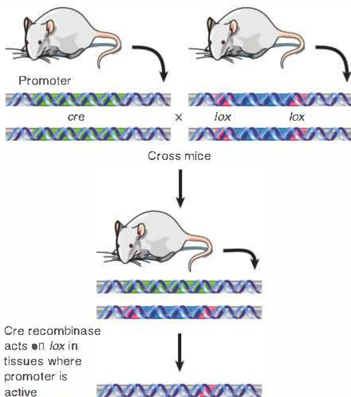
FIGURE 3.32 By placing the Cre recombinase under the control of a regulated promoter, it is possible to activate the excision system only in specific cells. One mouse is created that has a promoter- cre construct, and another that has a target sequence flanked by lox sites. The mice are crossed to generate progeny that have both constructs. Then excision of the target sequence can be triggered by activating the promoter.
