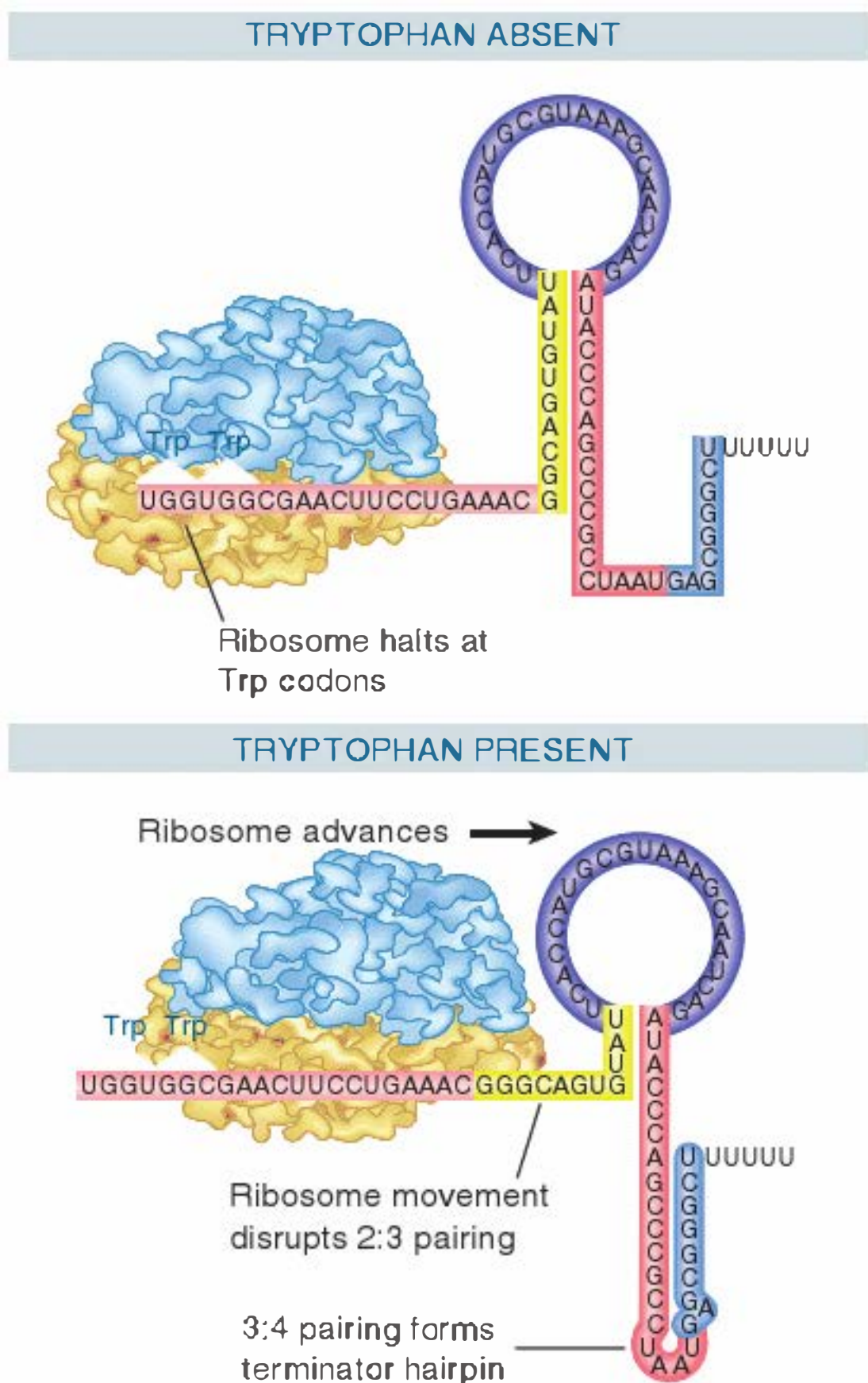
FIGURE 26.37 The alternatives for RNA polymerase at the attenuator depend on the location of the ribosome, which determines whether regions 3 and 4 can pair to form the terminator hairpin.
