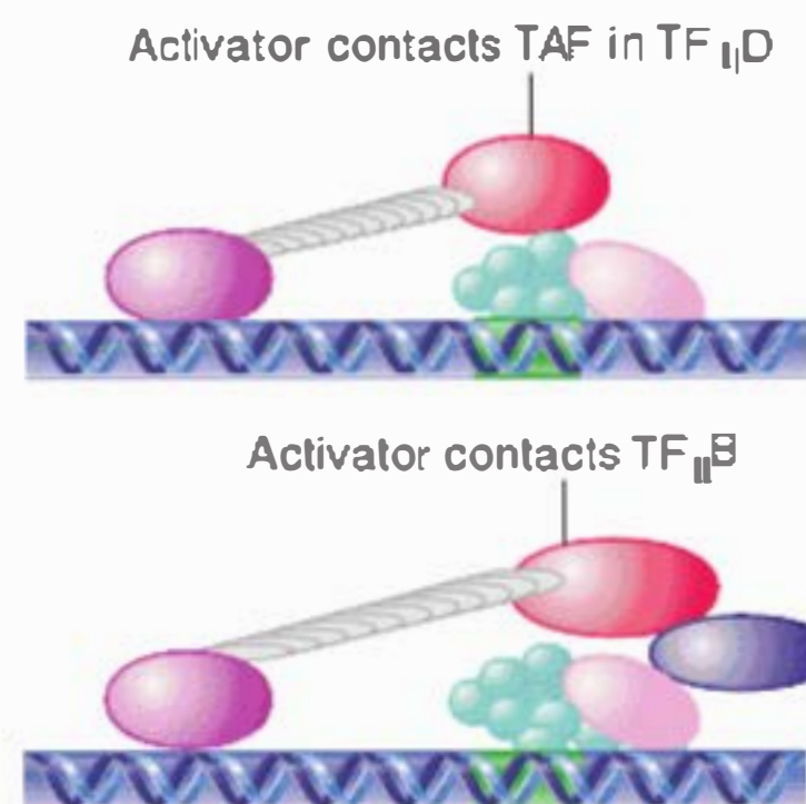
FIGURE 28.9 Activators may work at different stages of initiation by contacting the TAFs of TF IID or by contacting TF IIB .
